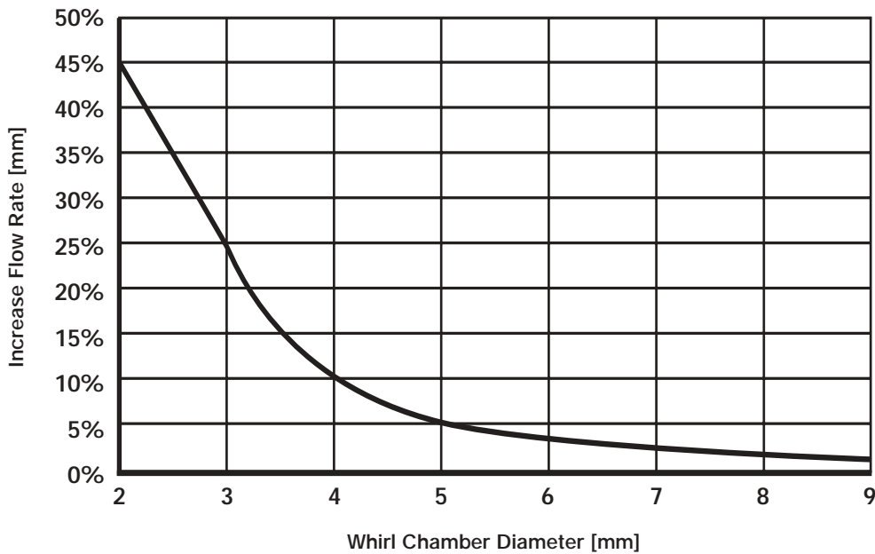
Increase Flow rate vs Whirl Chamber Diameter
